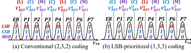
Figure 12: A comparison of (a) conventional V_{TH} state encoding and (b) proposed V_{TH} state encoding.
