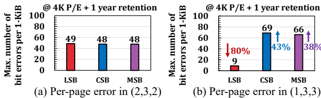
Figure 13: Impact of V_{TH} state encoding on page error rates.
